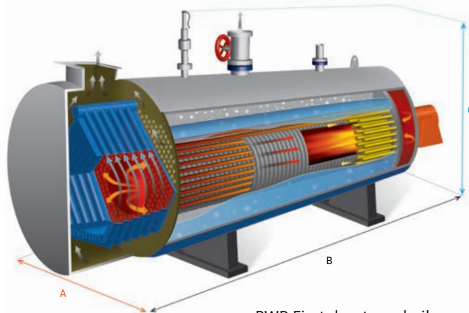
BWR Firetube steam boiler
