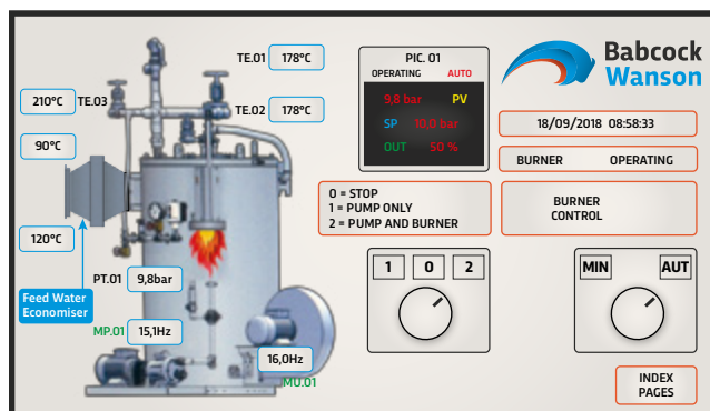
Fully modulating control with touch screen HMI
